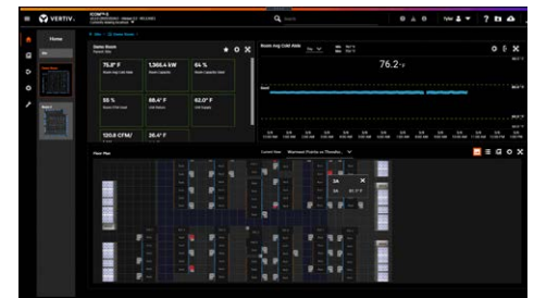
Room layout view with cold-aisle air properties
