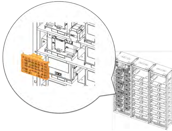
Figure 3-74: Reattach Module #11's Front Cover
