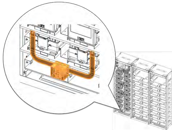
Figure 3-64: Connect Battery Module #8 B+ and Battery Module #9 B-.
