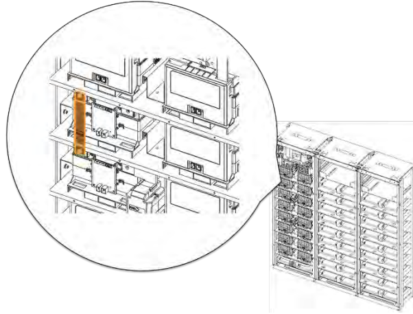
Figure 3-82: Connect Battery Module #14 B+ and Battery Module #15 B-.
