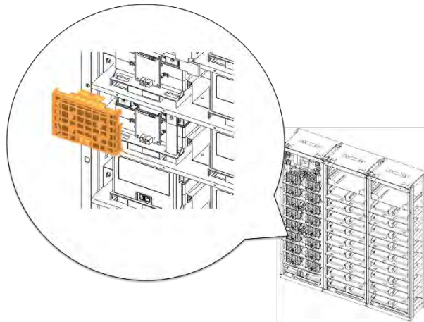
Figure 3-69: Remove Battery Module #11's Front Cover
