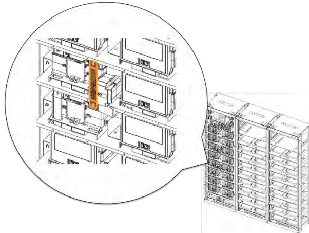
Figure 3-73: Connect Battery Module #11 B+ and Battery Module #12 B-.
