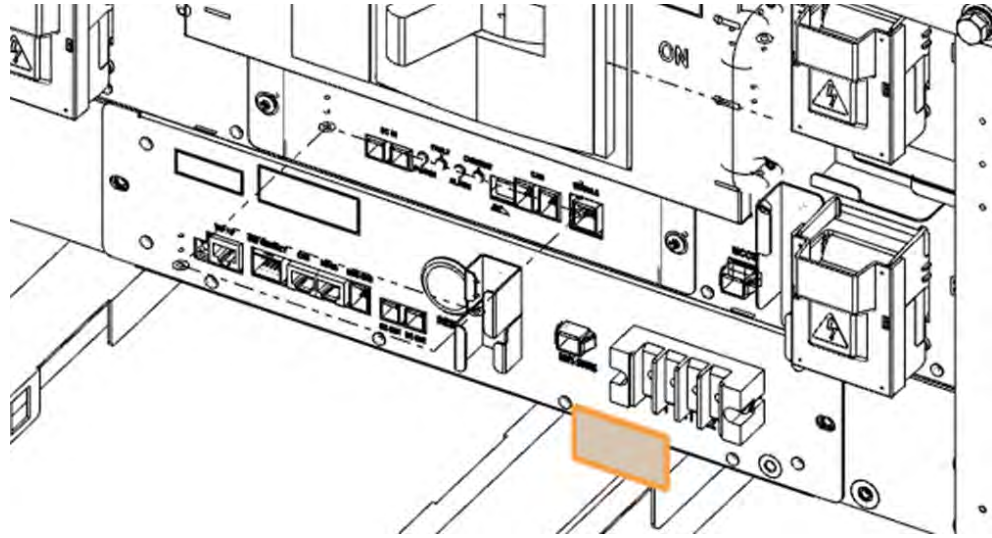
Figure 3-117: AC Input Terminals of SMPS Assembly 1 Phase Type A
