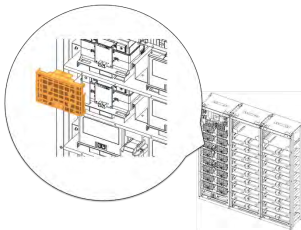
Figure 3-84: Remove Battery Module #16's Front Cover
