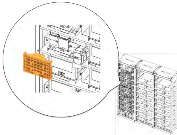
Figure 3-83: Reattach Battery Module #14's Front Cover
