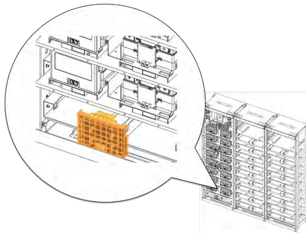
Figure 3-60: Remove Battery Module #8's Front Cover
