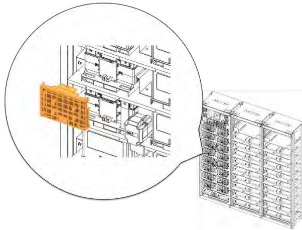
Figure 3-75: Remove Module #13's Front Cover
