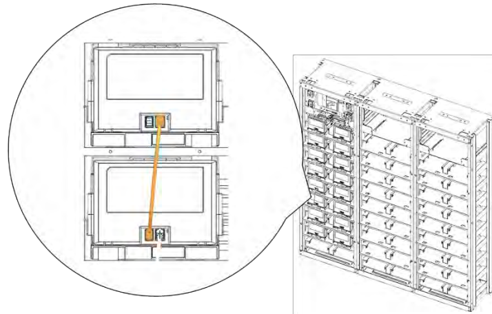
Figure 3-101: Module #11 to Module #12 Signal Cabling
