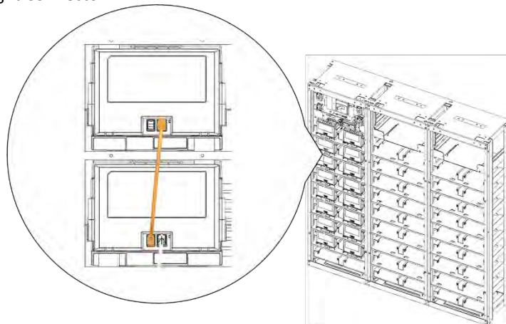
Figure 3-104: Module #14 to Module #15 Signal Cabling
