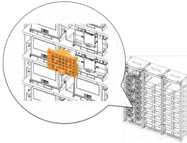
Figure 3-59: Reattach Battery Module #6's Front Cover
