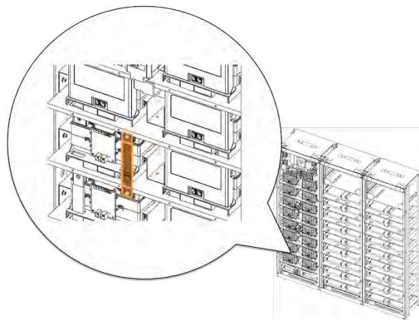
Figure 3-67 Connect Battery Module #9 B+ and Battery Module #10 B-.
