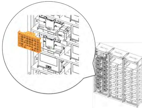
Figure 3-72: Remove Battery Module #12's Front Cover
