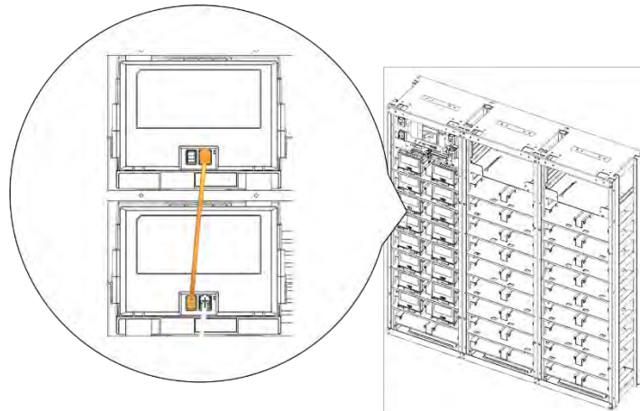
Figure 3-103: Module #13 to Module #14 Signal Cabling
