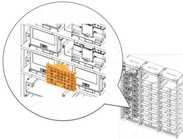
Figure 3-57: Remove Battery Module #7's Front Cover
