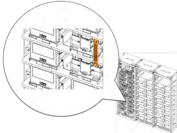
Figure 3-58: Connect Battery Module #6 B+ and Battery Module #7 B-
