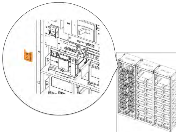
Figure 3-87: Remove SMU B+ Terminal Cover
