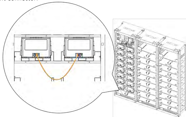
Figure 3-98: Module #8 to Module #9 Signal Cabling
