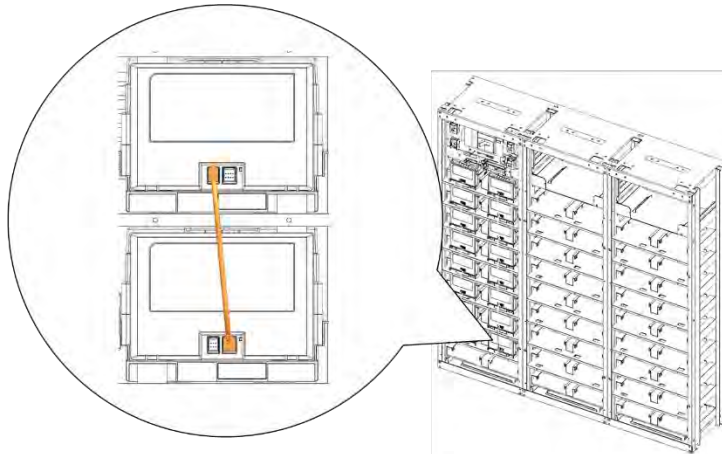
Figure 3-97: Module #7 to Module #8 Signal Cabling
