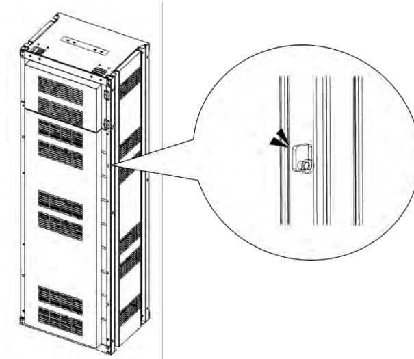
Figure 3-131: Front panel hooks (four)
