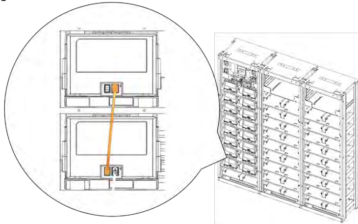
Figure 3-99: Module #9 to Module #10 Signal Cabling
