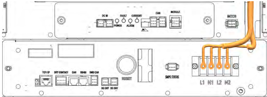
Figure 3-121: SMPS Assembly 1 Phase Type A - AC Input Terminals with Cables Attached
