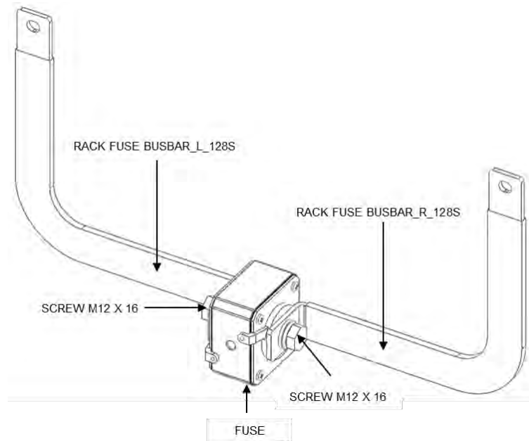
Figure 3-30: Rack Fuse Busbar Assembly
