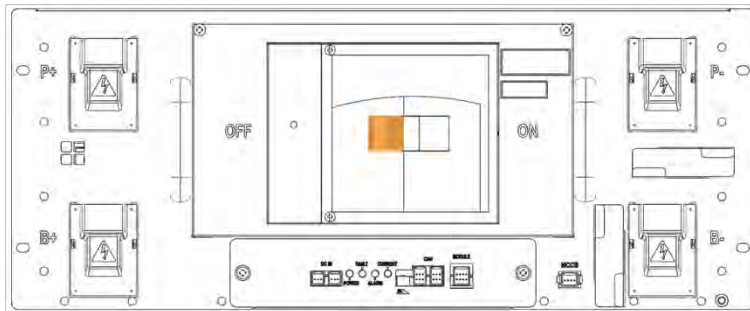
Figure 3-134: MCCB Handle in Off Position
