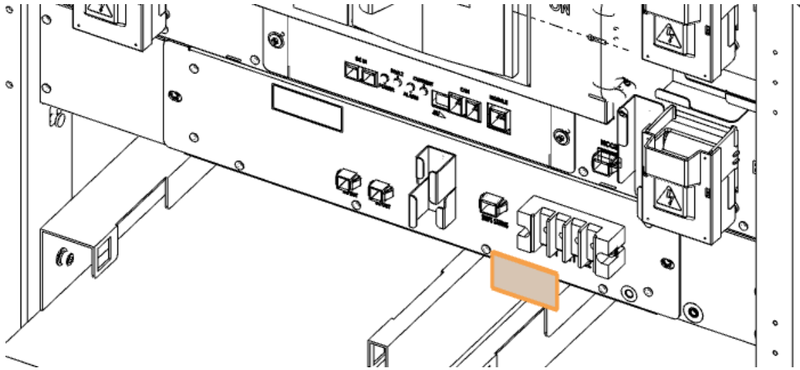
Figure 3-126: AC Input Terminals of SMPS Assembly 1 Phase Type B
