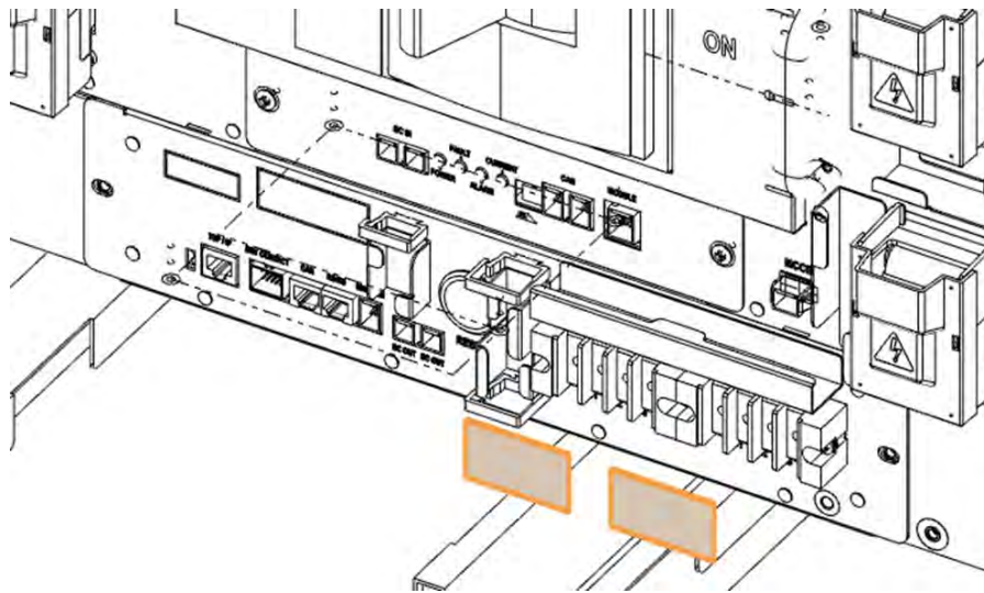
Figure 3-123: AC Input Terminals of SMPS Assembly 3 Phase Type A
