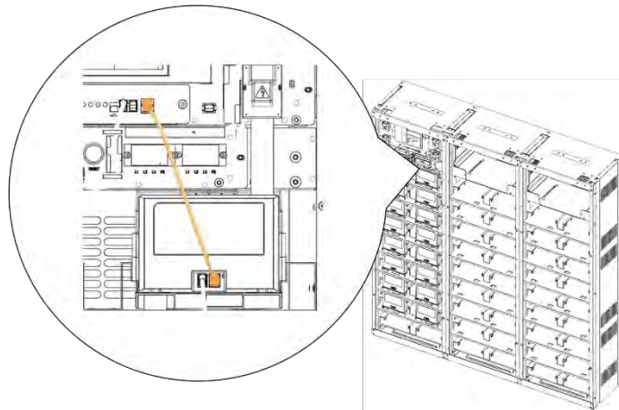
Figure 3-90: SMU to Module #1 Signal Cable
