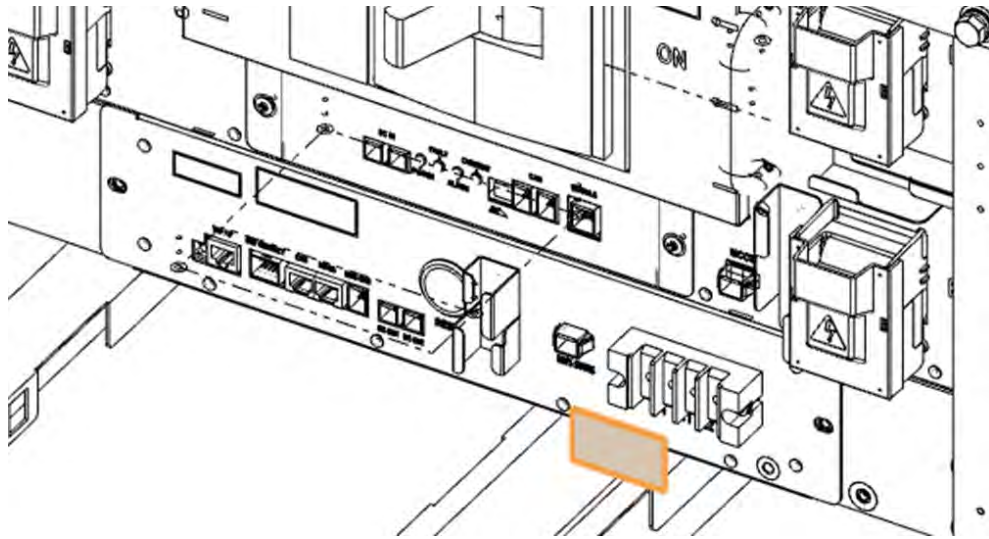
Figure 3-125: AC Input Terminals of SMPS Assembly 1 Phase Type A
