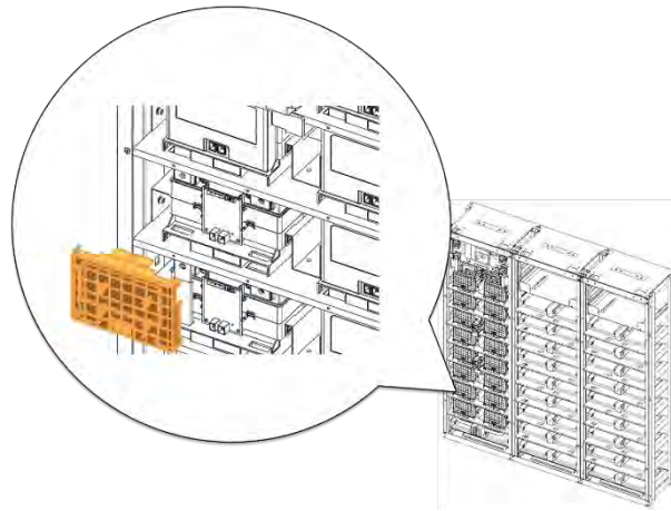
Figure 3-66: Remove Battery Modules #10's Front Cover
