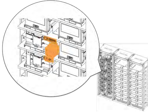
Figure 3-79: Connect Battery Module #13 B+ and Battery Module #14 B-.
