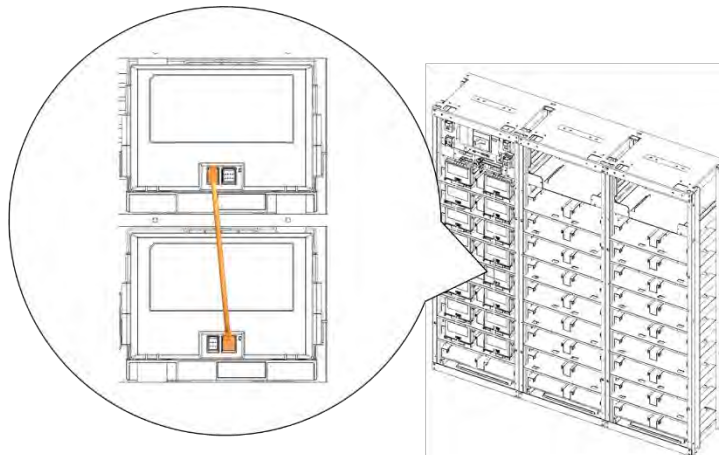
Figure 3-94: Module #4 to Module #5 Signal Cabling
