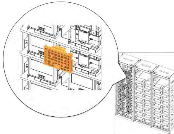
Figure 3-44: Reattach Battery Module #1's Front Cover
