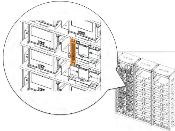
Figure 3-49: Connect Battery Module #3 B+ and Module #4 B-.
