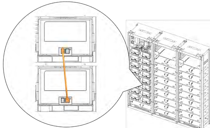
Figure 3-95: Module #5 to Module #6 Signal Cabling
