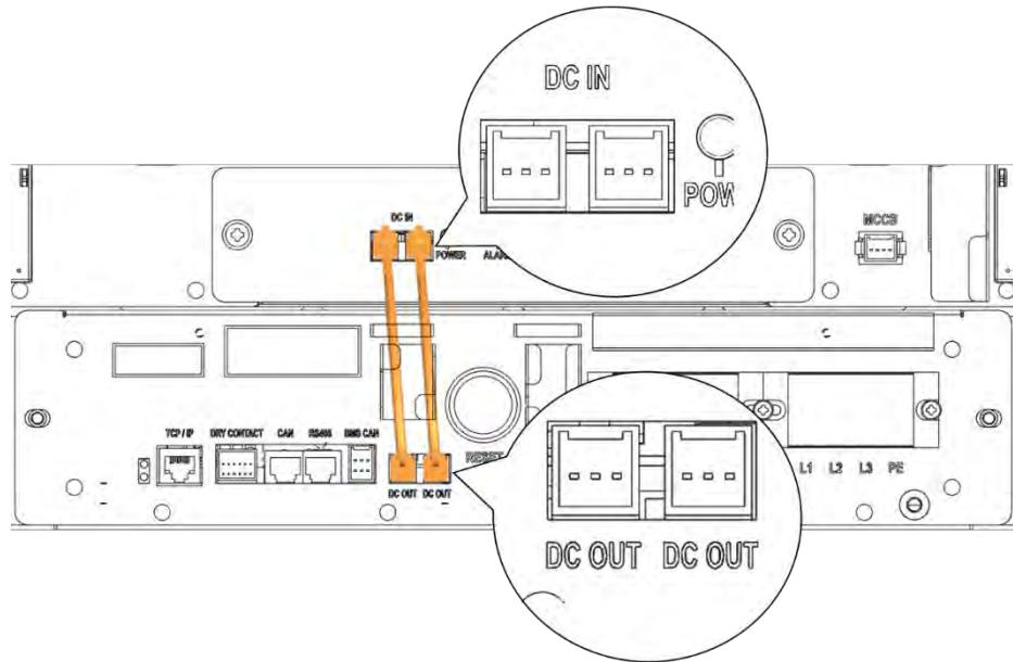
Figure 3-109: DC Power Cables from SMPS Assembly 3 Phase Type A to SMU
