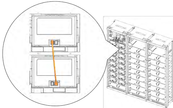
Figure 3-91: Module #1 to Module #2 Signal Cabling
