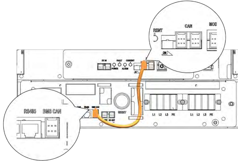
Figure 3-111: CAN Signal Cable Connection from SMPS Assembly 3 Phase Type A to SMU
