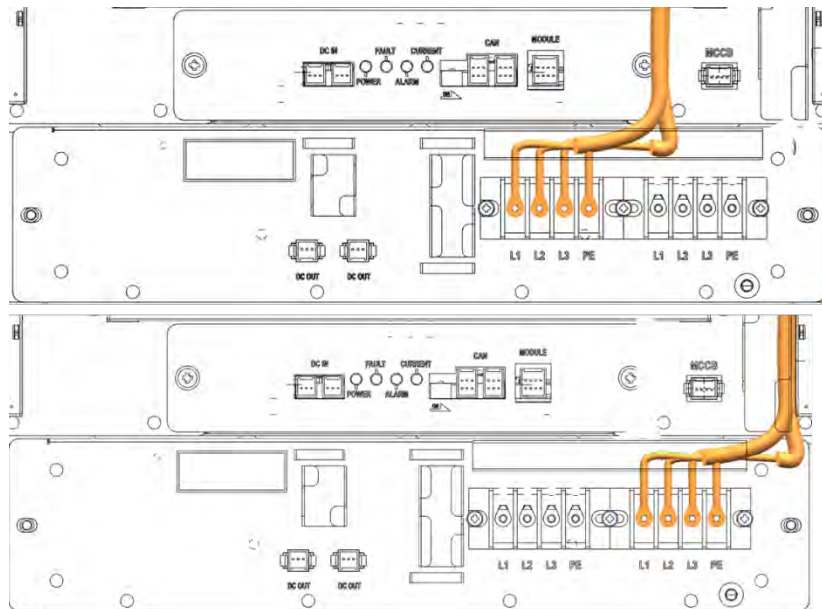
Figure 3-120: SMPS Assembly 3 Phase Type B - AC Input Terminals with Cables Attached
