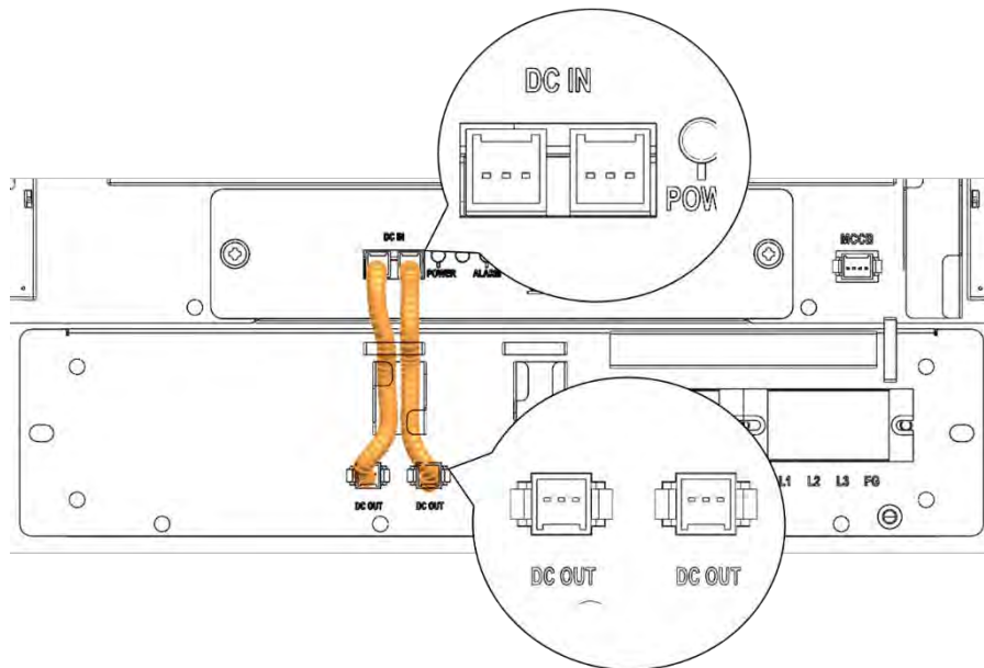
Figure 3-110: DC Power Cables from SMPS Assembly 3 Phase Type B to SMU
