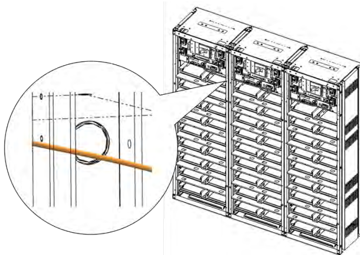
Figure 3-106: Pre-Punched Hole for Signal Cable
