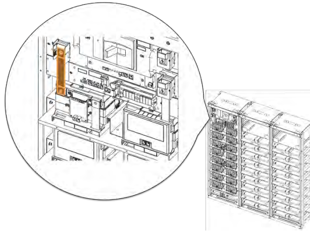
Figure 3-88: Connect SMU B+ and Module #16 B+.
