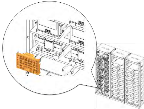
Figure 3-63: Remove Battery Modules #9's Front Cover
