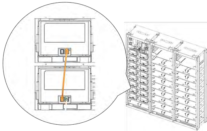
Figure 3-100: Module #10 to Module #11 Signal Cabling
