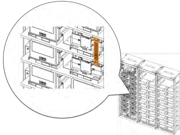
Figure 3-52: Connect Battery Module #4 B+ and Battery Module #5 B-.
