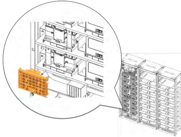
Figure 3-68: Reattach Battery Module #9's Front Cover
