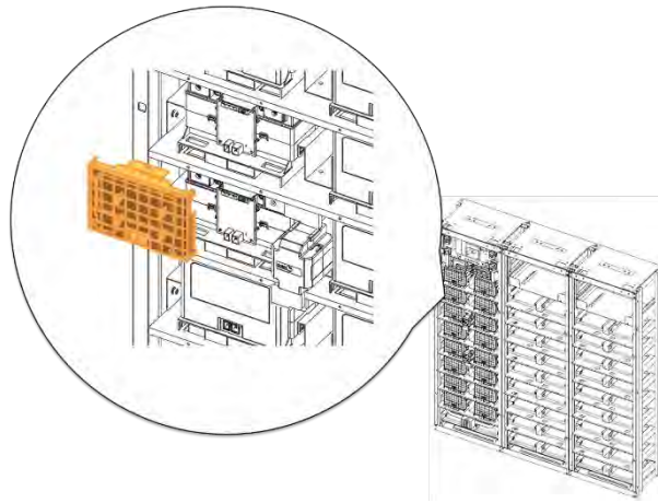
Figure 3-81: Remove Battery Module #15's Front Cover
