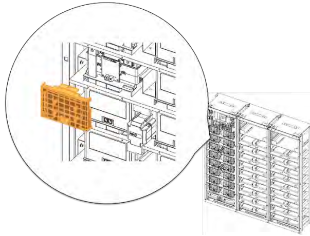
Figure 3-86: Reattach Battery Module #15's Front Cover
