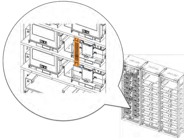
Figure 3-61: Connect Battery Module #7 B+ and Battery Module #8 B-
