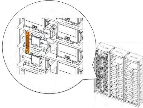
Figure 3-70: Connect Battery Module #10 B+ and Battery Module #11 B-.
