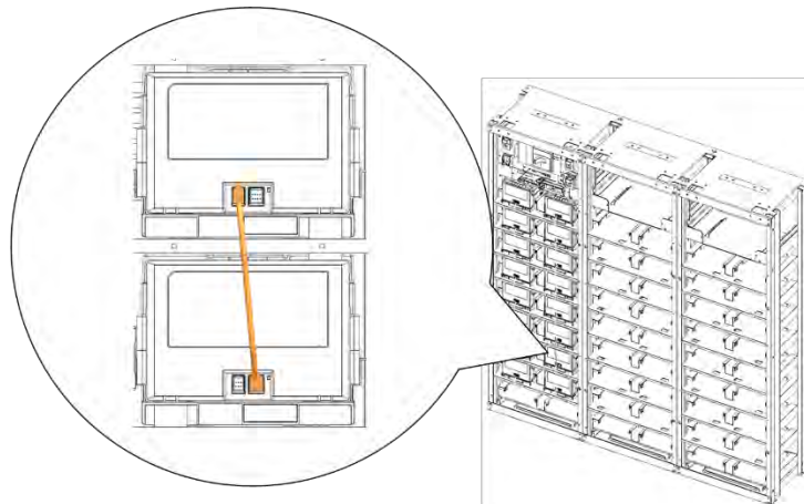
Figure 3-96: Module #6 to Module #7 Signal Cabling
