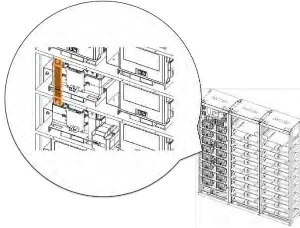
Figure 3-76: Connect Battery Module #12B+ and Battery Module #13 B-.
