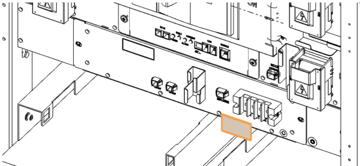
Figure 3-118: AC Input Terminals of SMPS Assembly 1 Phase Type B
