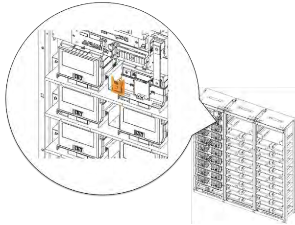
Figure 3-41: Restore SMU's B- Terminal
