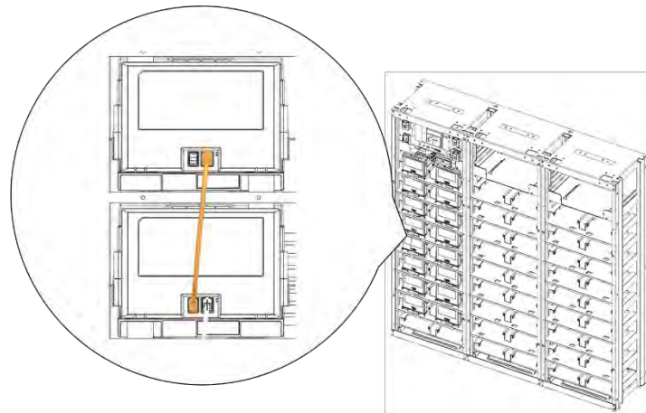
Figure 3-102: Module #12 to Module #13 Signal Cabling
