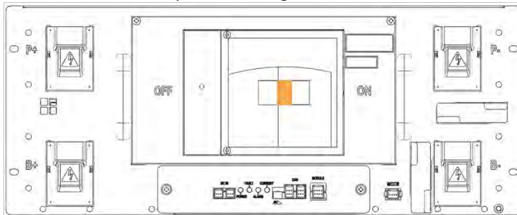
Figure 3-133: MCCB Handle in Trip Position
