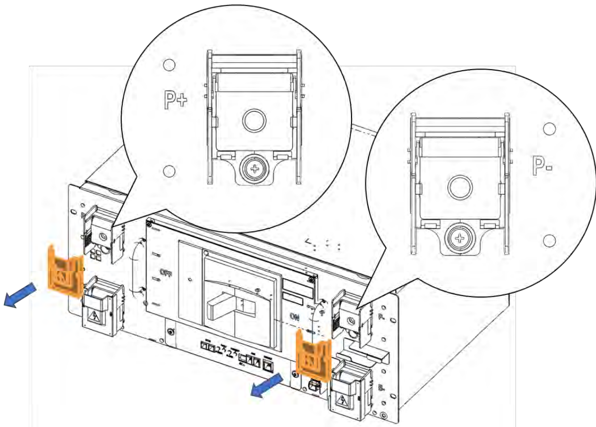
Figure 3-128: Connecting the DC Link High Current Terminals
