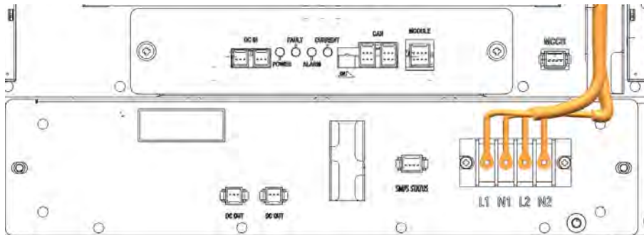
Figure 3-122: SMPS Assembly 1 Phase Type B - AC Input Terminals with Cables Attached
