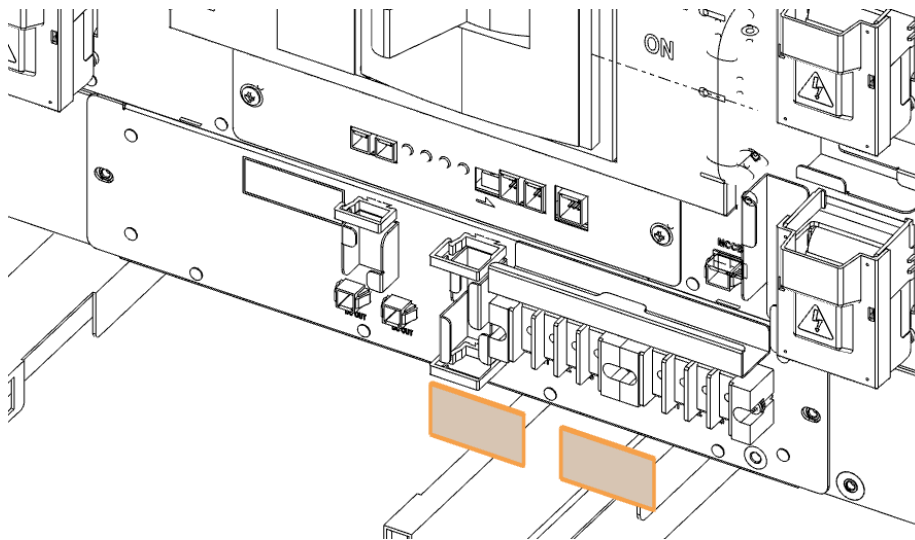
Figure 3-116: AC Input Terminals of SMPS Assembly 3 Phase Type B
