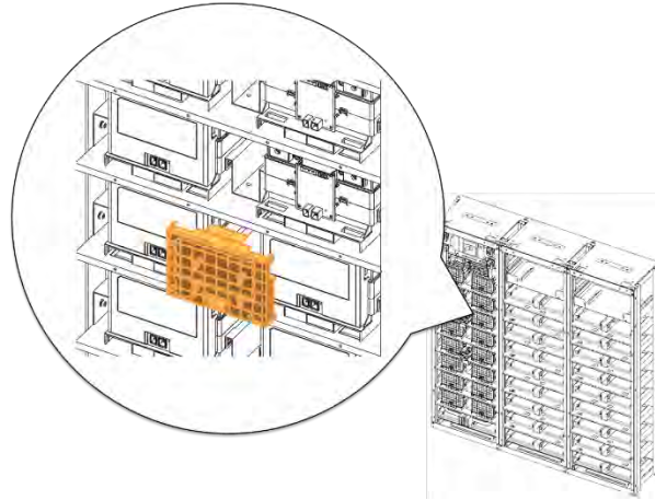
Figure 3-45: Remove Battery Module #2's Front Cover
