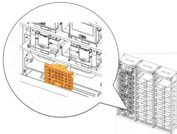
Figure 3-65: Reattach Battery Modules #8's Front Cover
