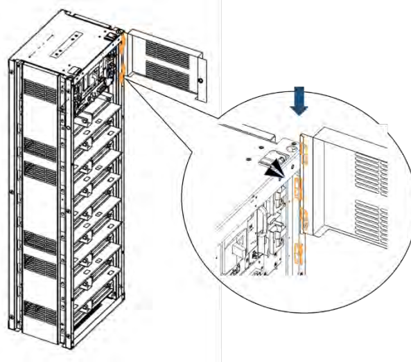
Figure 3-129: Reattaching the Front Door
