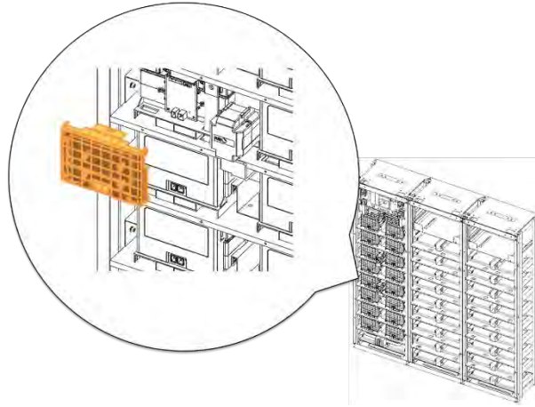
Figure 3-77: Reattach Module #12's Front Cover
