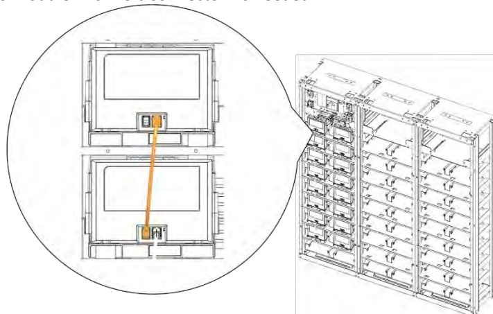
Figure 3-105: Module #15 to Module #16 Signal Cabling
