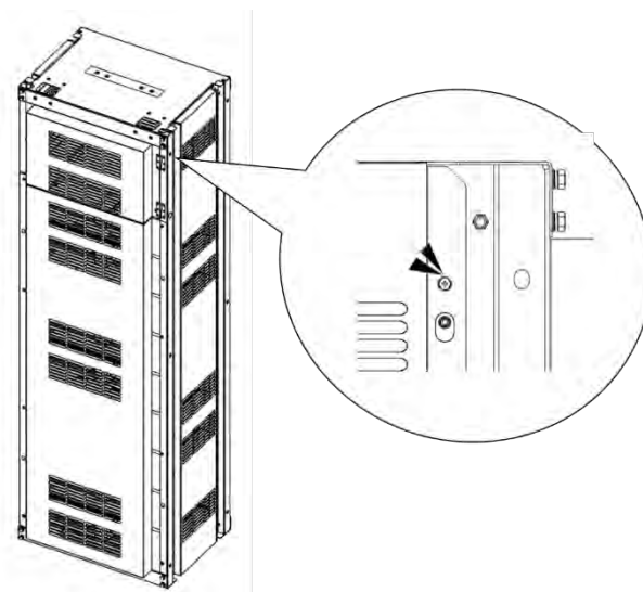
Figure 3-7: Side panel screws (six)
