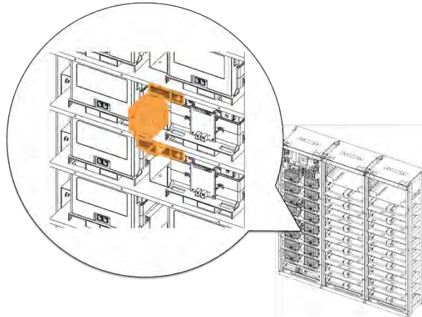
Figure 3-55: Connect Battery Module #5 B+ and Battery Module #6 B-.
