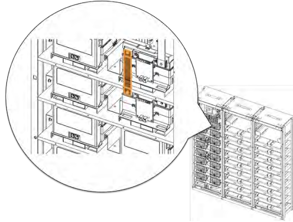
Figure 3-43: Connect Battery Module #1 B+ and Battery Module #2 B-.
