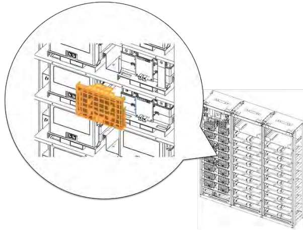
Figure 3-53: Reattach Battery Module #4's Front Cover
