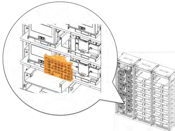
Figure 3-62: Reattach Battery Modules #7's Front Cover
