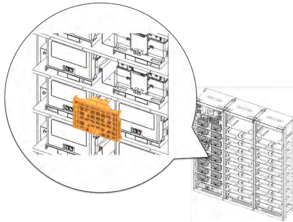
Figure 3-51: Remove Battery Module #5's Front Cover
