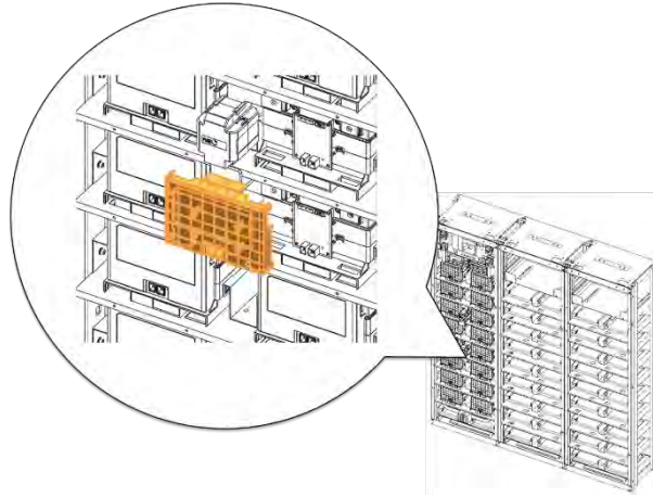
Figure 3-56: Reattach Battery Module #5's Front Cover
