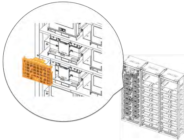
Figure 3-78: Remove Battery Module #14's Front Cover
