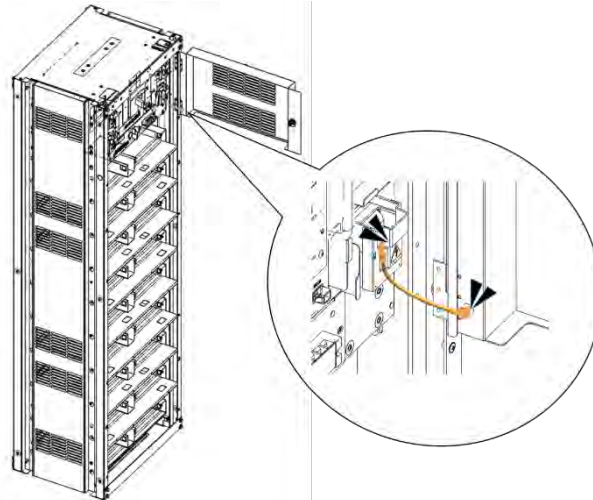
Figure 3-130: Reattaching the earth cable.
