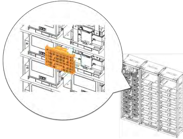
Figure 3-50: Reattach Battery Module #3's Front Cover
