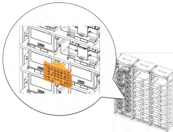
Figure 3-54: Remove Battery Module #6's Front Cover
