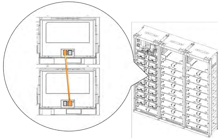
Figure 3-93: Module #3 to Module #4 Signal Cabling
