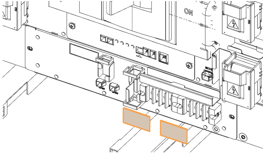
Figure 3-124: AC Input Terminals of SMPS Assembly 3 Phase Type B
