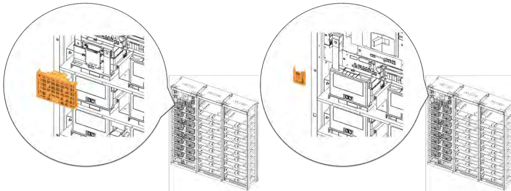
Figure 3-89: Reattach Battery Module #16's Front Cover and SMU B+ Terminal Cover
