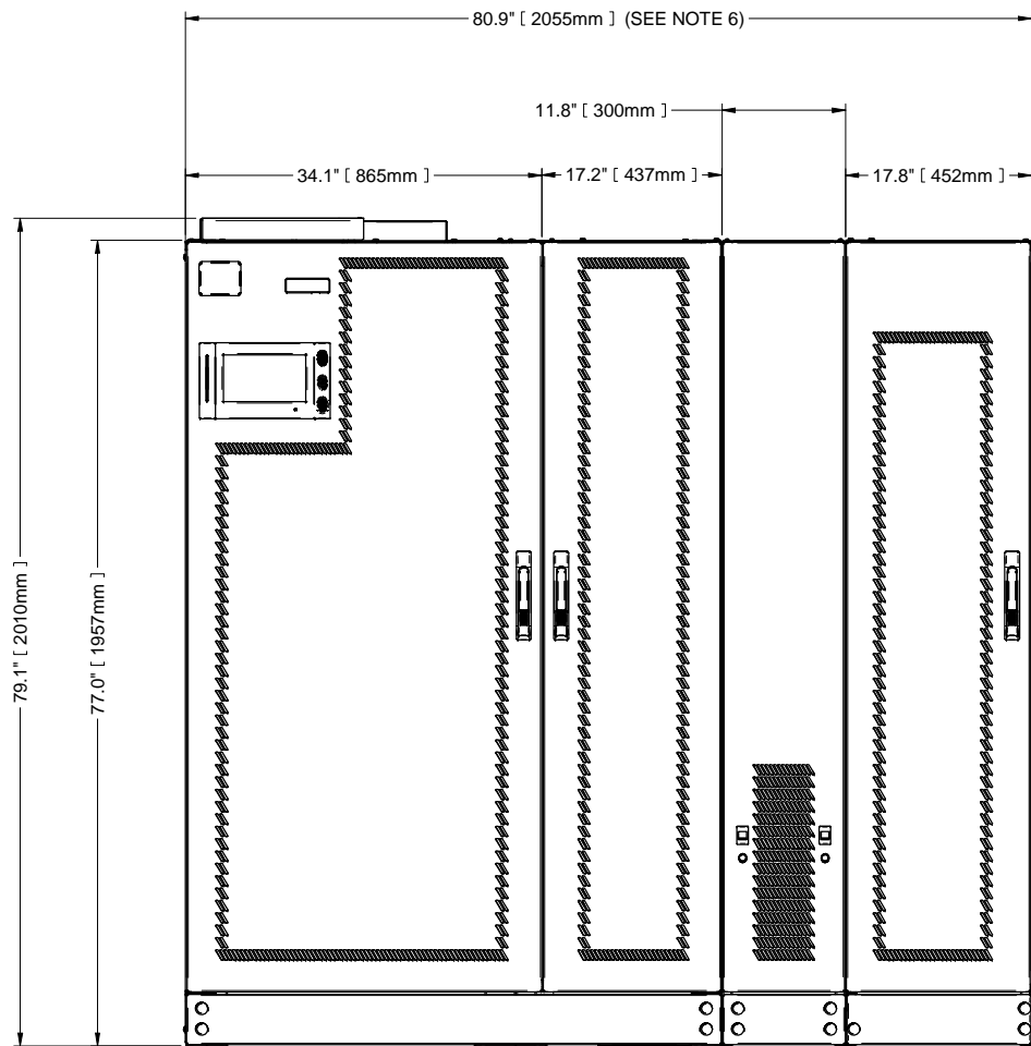
FRONT VIEW
